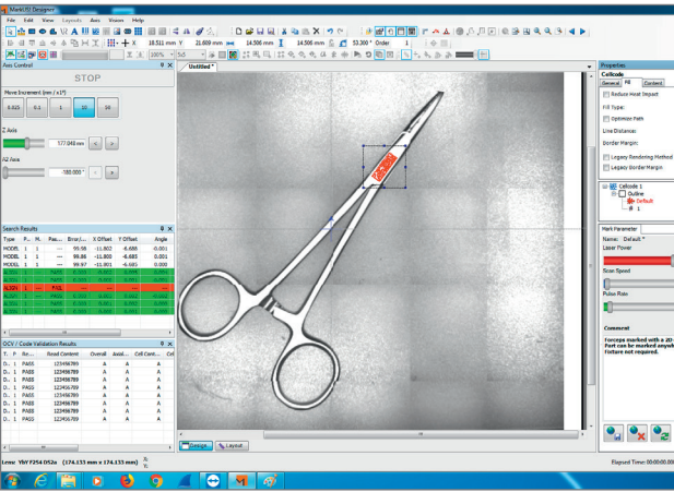
Mosaic™ is trained to validate the part (green results) and align a laser mark on a pair of forceps. Although the part is randomly placed under the laser, the system is capable of aligning the mark to the part.
